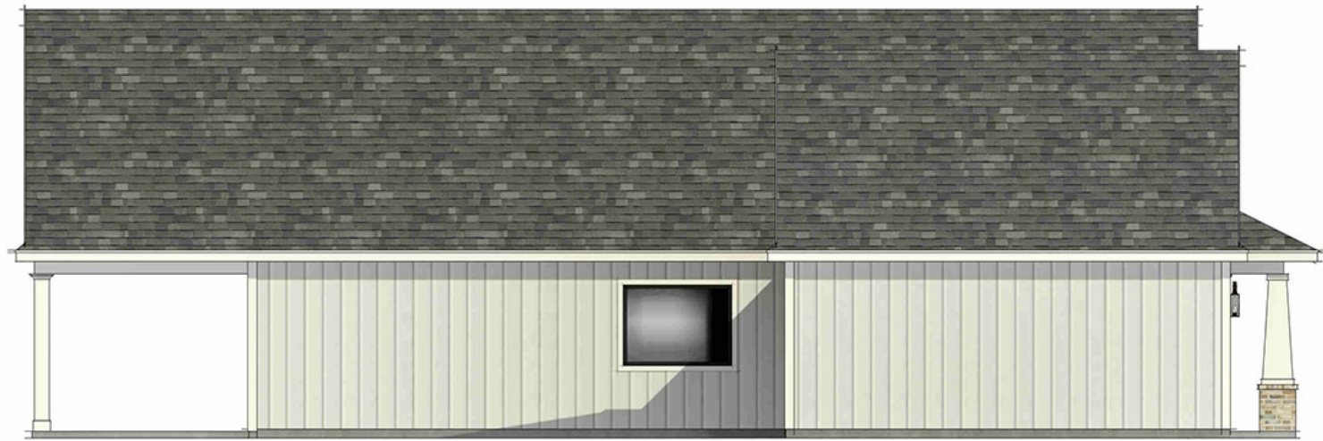
LEFT ELEVATION
